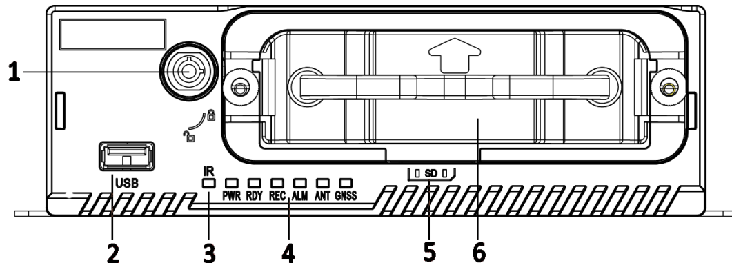
Front Panel
